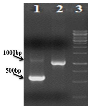
Figure 1. Cloning of IFNγ-bar fusion in pCAMBIA1305.1 expression vector. The IFNγ-bar has been cloned between the SpeI and BstEII restriction sites and downstream of the catalase intron
